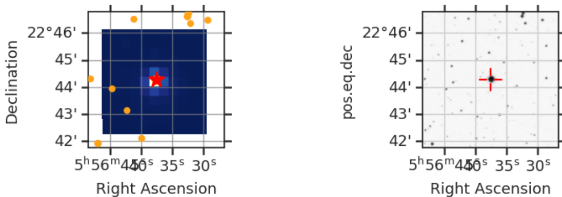
Fig 7. The locations of nearby GAIA DR2 stars with a magnitude difference less than 5 (orange circle) within the Tess Cut Out around TIC 119180868 (red star). Only shown for one sector. Right: SDSS image of the surrounding field.
