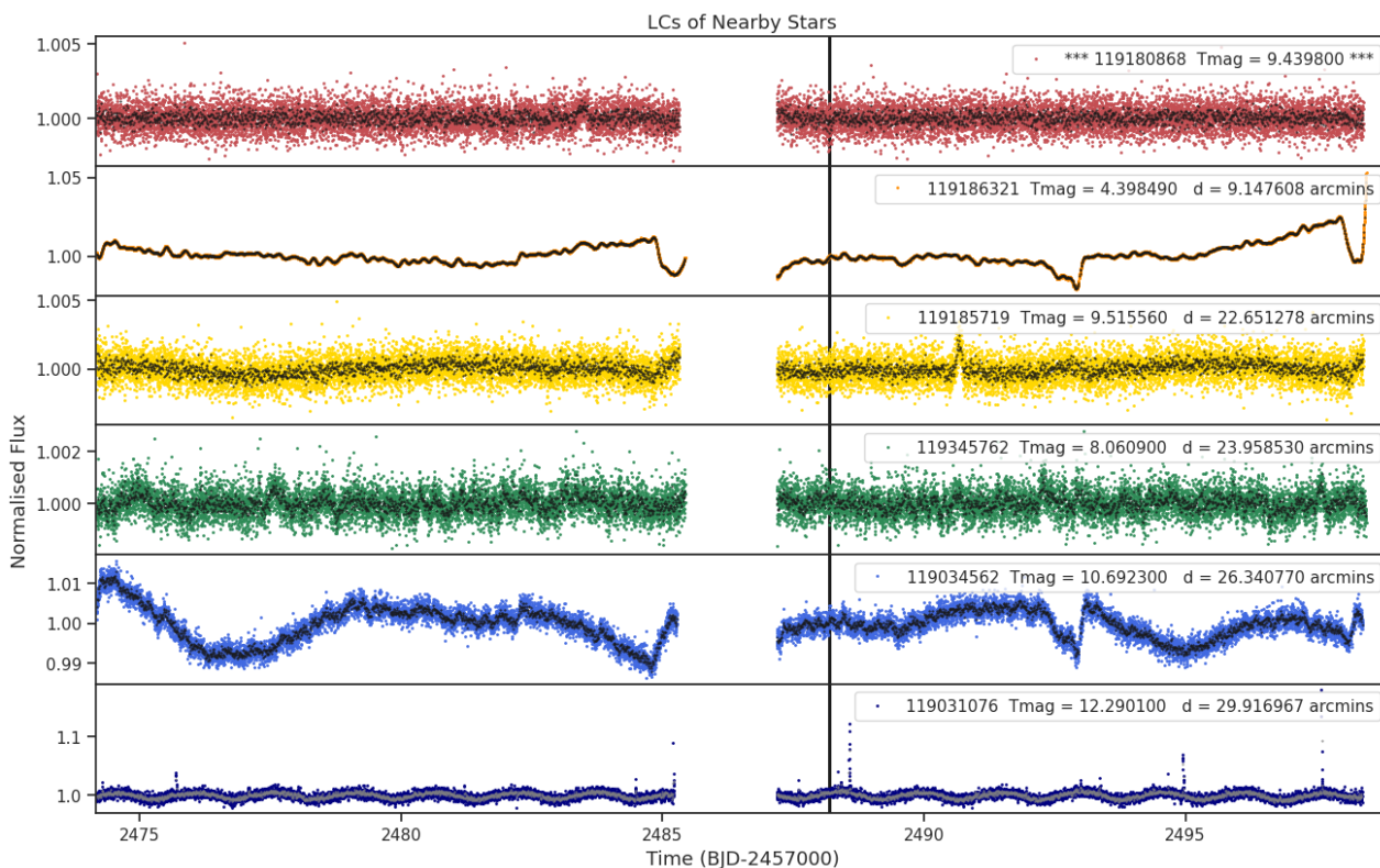
Fig 8. Lightcurves of the five closest stars to target 119180868 (top panel). The distances to the target star and the TESS magnitudes are shown for each star. Only ever shown for one sector.
