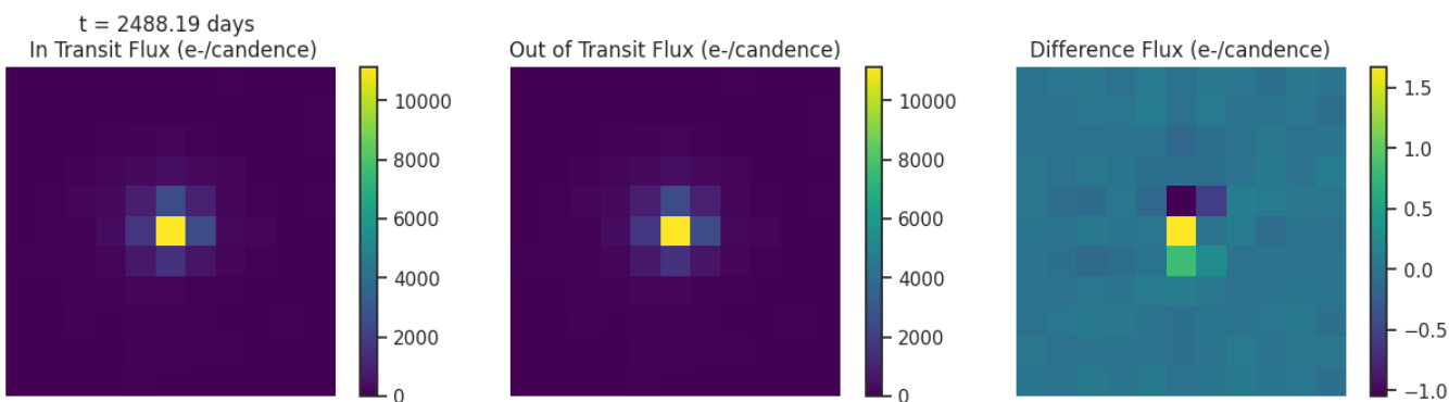
Fig 6. Difference images for target TIC 119180868 for each transit like event. Left: mean in-transit flux(left). Middle: mean out-of-transit flux. Right: difference between the mean out-of-transit and mean in-transit flux. Ensure that the change in brightness occurs on target.
