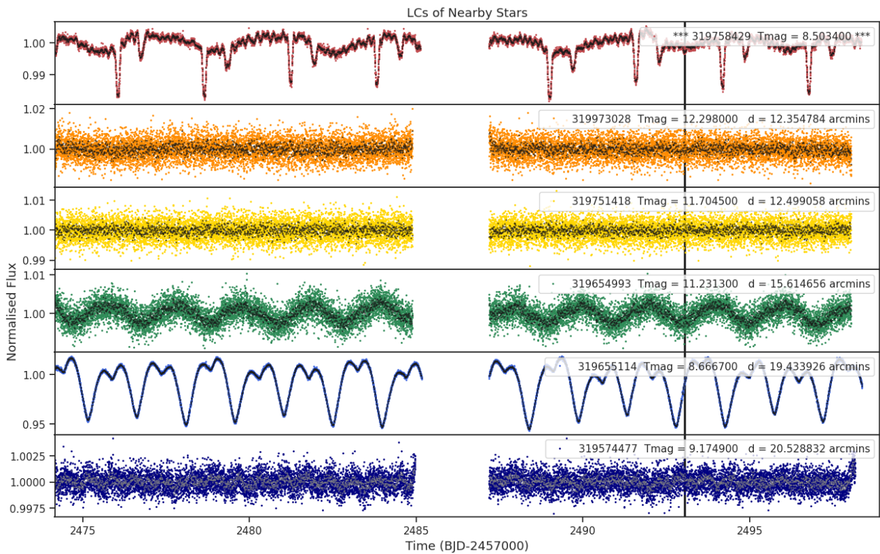
Fig 8. Lightcurves of the five closest stars to target 319758429 (top panel). The distances to the target star and the TESS magnitudes are shown for each star. Only ever shown for one sector.
