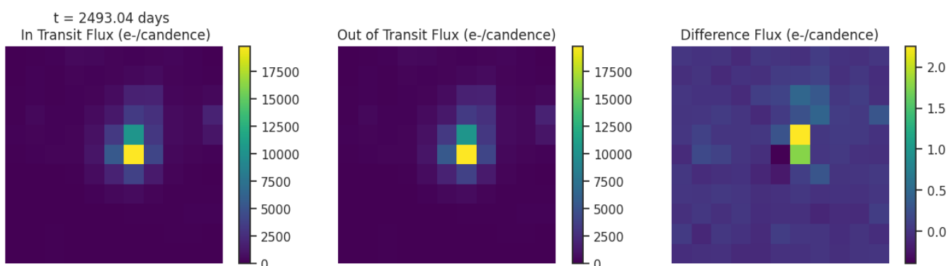
Fig 6. Difference images for target TIC 319758429 for each transit like event. Left: mean in-transit flux(left). Middle: mean out-of-transit flux. Right: difference between the mean out-of-transit and mean in-transit flux. Ensure that the change in brightness occurs on target.
