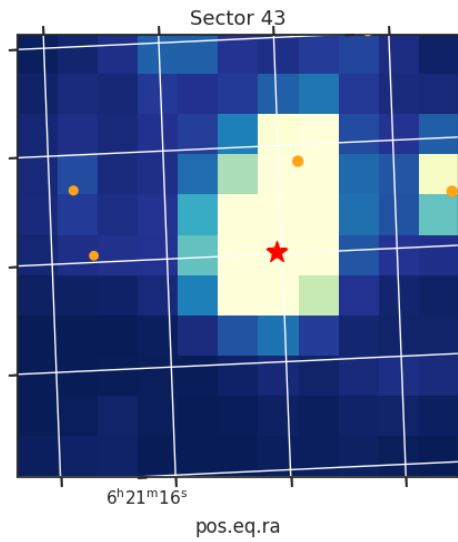
Fig 7. The locations of nearby GAIA DR2 stars with a magnitude difference less than 5 (orange circle) within the Tess Cut Out around TIC 319758429 (red star). Only shown for one sector. Right: SDSS image of the surrounding field.
