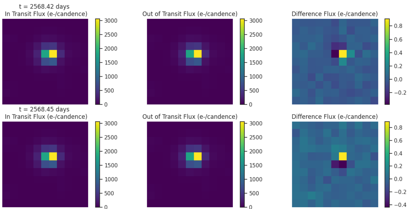
Fig 6. Difference images for target TIC 32481343 for each transit like event. Left: mean in-transit flux(left). Middle: mean out-of-transit flux. Right: difference between the mean out-of-transit and mean in-transit flux. Ensure that the change in brightness occurs on target.
