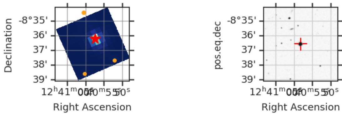
Fig 7. The locations of nearby GAIA DR2 stars with a magnitude difference less than 5 (orange circle) within the TESS Cut Out around TIC 32481343 (red star). Only shown for one sector. Right: SDSS image of the surrounding field.
