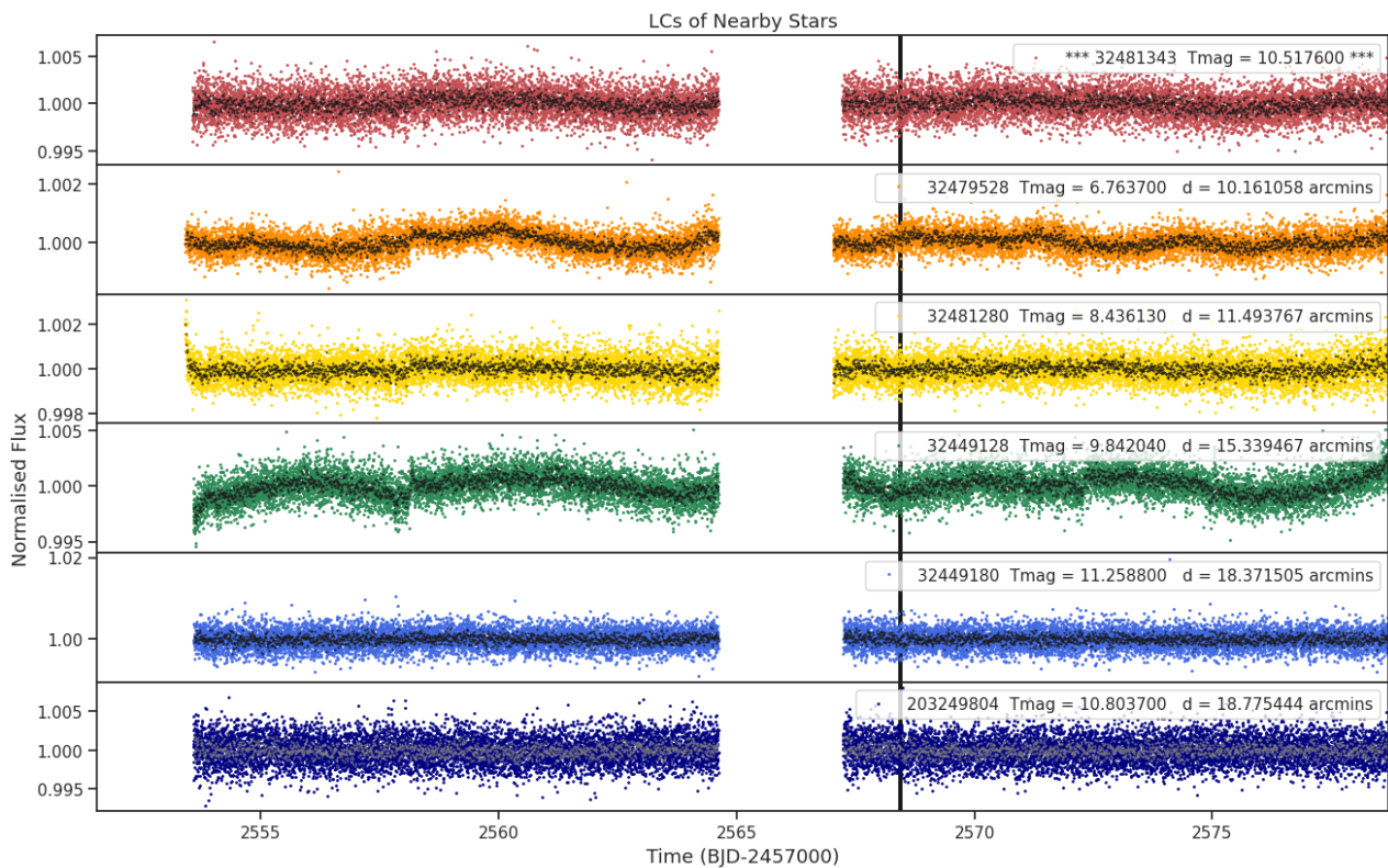
Fig 8. Lightcurves of the five closest stars to target 32481343 (top panel). The distances to the target star and the TESS magnitudes are shown for each star. Only ever shown for one sector.
