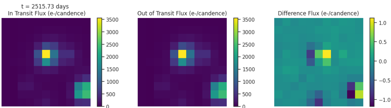
Fig 6. Difference images for target TIC 337385330 for each transit like event. Left: mean in-transit flux(left). Middle: mean out-of-transit flux. Right: difference between the mean out-of-transit and mean in-transit flux. Ensure that the change in brightness occurs on target.
