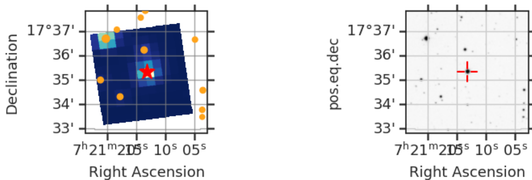
Fig 7. The locations of nearby GAIA DR2 stars with a magnitude difference less than 5 (orange circle) within the Tess Cut Out around TIC 337385330 (red star). Only shown for one sector. Right: SDSS image of the surrounding field.
