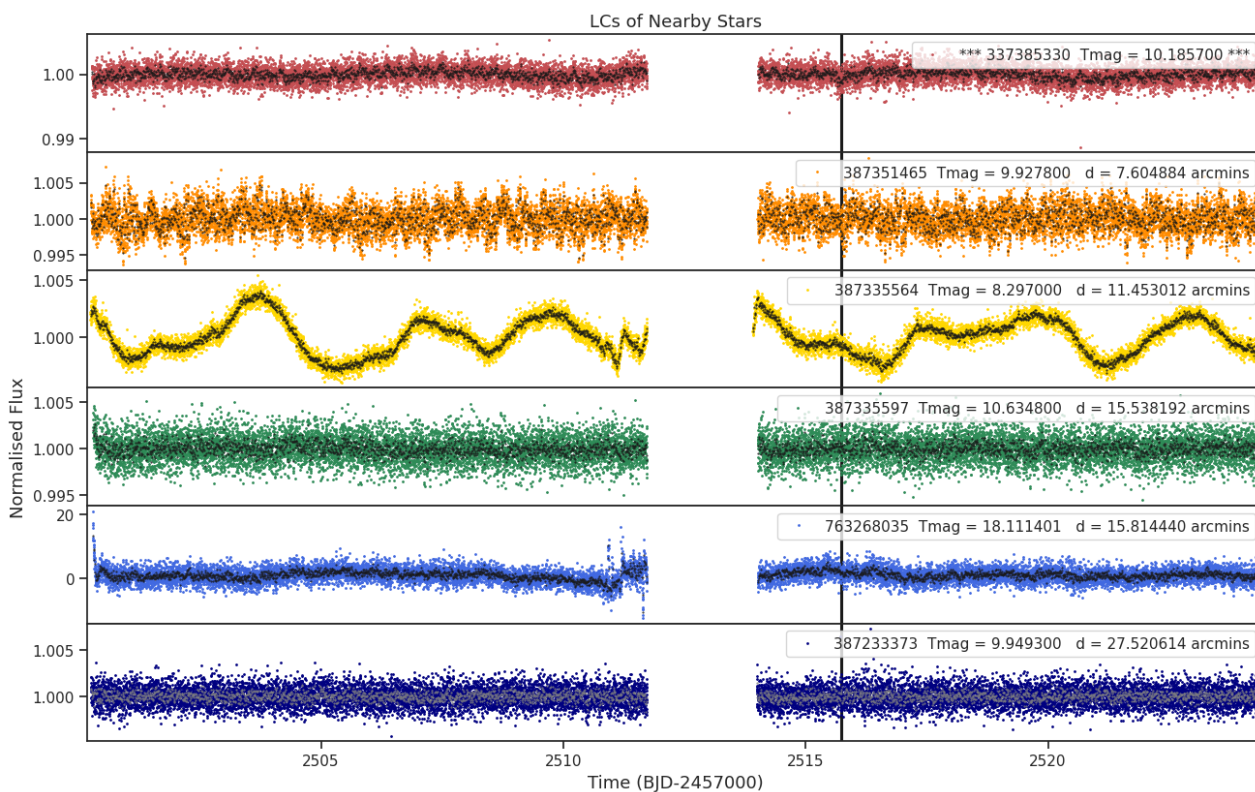
Fig 8. Lightcurves of the five closest stars to target 337385330 (top panel). The distances to the target star and the TESS magnitudes are shown for each star. Only ever shown for one sector.
