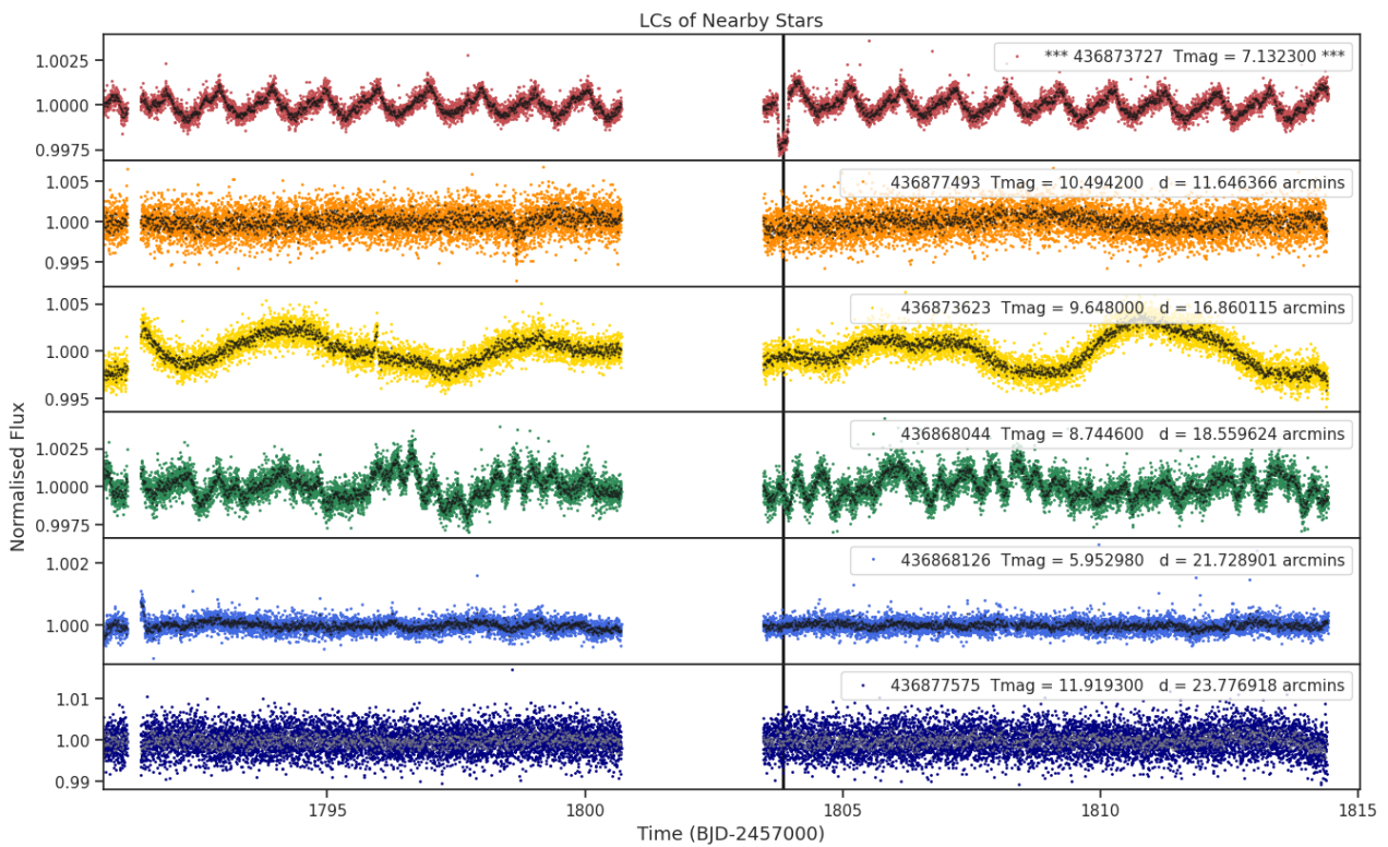
Fig 8. Lightcurves of the five closest stars to target 436873727 (top panel). The distances to the target star and the TESS magnitudes are shown for each star. Only ever shown for one sector.
