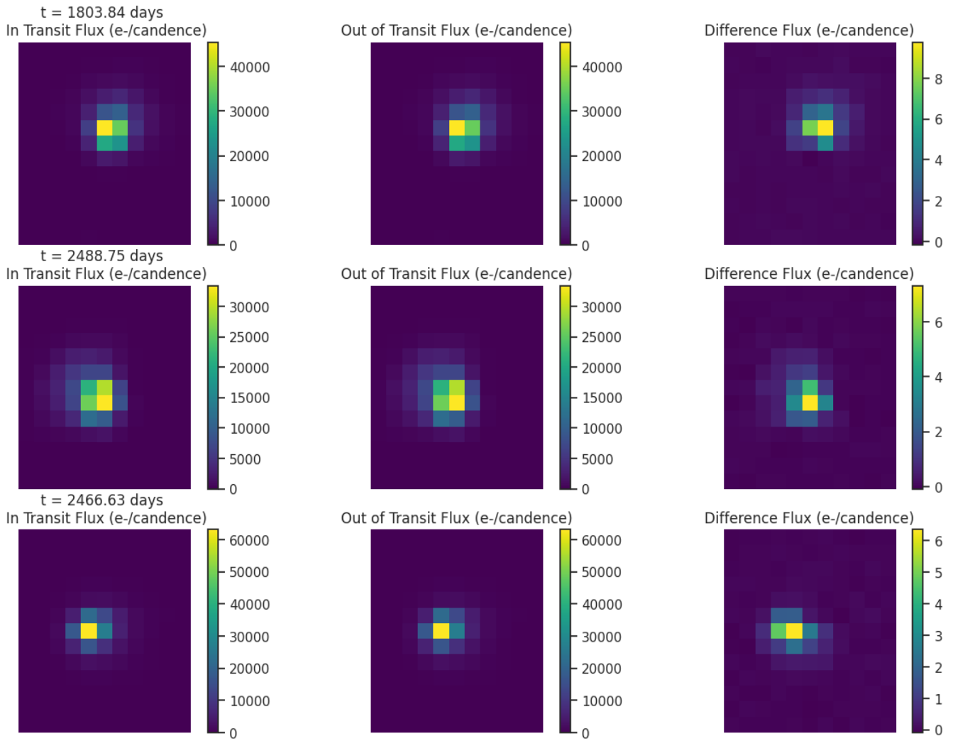
Fig 6. Difference images for target TIC 436873727 for each transit like event. Left: mean in-transit flux(left). Middle: mean out-of-transit flux. Right: difference between the mean out-of-transit and mean in-transit flux. Ensure that the change in brightness occurs on target.
