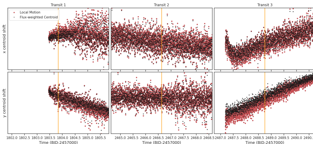
Fig 3. The x and y centroid positions around the time of each transit-like event. The black points shows the CCD column and row position of the target's flux-weighted centroid. The red shows the CCD column and row local motion differential velocity aberration (DVA), pointing drift, and thermal effects. The vertical orange line indicates the time of the transit-like event
