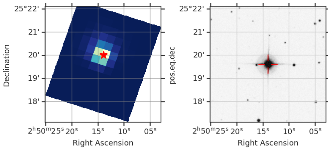
Fig 7. The locations of nearby GAIA DR2 stars with a magnitude difference less than 5 (orange circle) within the TESS Cut Out around TIC 436873727 (red star). Only shown for one sector. Right: SDSS image of the surrounding field.
