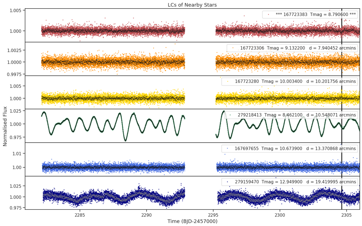
Fig 8. Lightcurves of the five closest stars to target 167723383 (top panel). The distances to the target star and the TESS magnitudes are shown for each star. Only ever shown for one sector.
