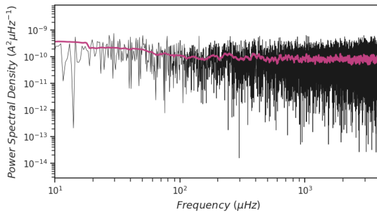
Fig 10. Lomb scargle power spectrum of the TESS lightcurve (black line) and a boxcar-smoothed periogram (pink line) computed with a window length of 20 micro Hz.
