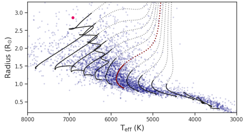
Fig 11. The equivalent evolutionary phase (eep) tracks for main sequence evolution (solid lines) and post main-sequence evolution (dashed lines) for masses ranging from 0.3 to 1.6 solar masses (from right to left). The 1 Solar Mass track is shown in maroon. The blue points show the TOIs and the magenta point TIC 167723383.
