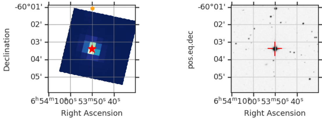
Fig 7. The locations of nearby GAIA DR2 stars with a magnitude difference less than 5 (orange circle) within the Tess Cut Out around TIC 167723383 (red star). Only shown for one sector. Right: SDSS image of the surrounding field.
